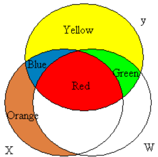
Figure 3b Considerable collinearity
