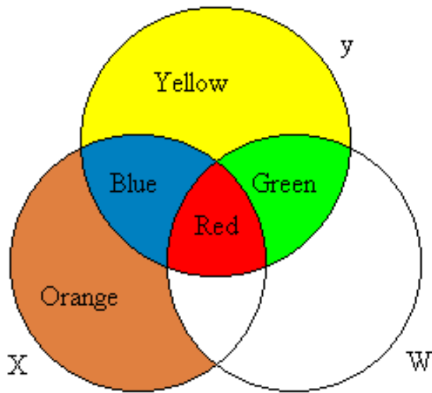
Figure 3a Modest collinearity
